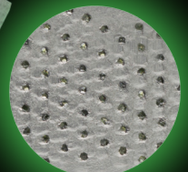
Close-Up of Organized Diamonds in the Segment
