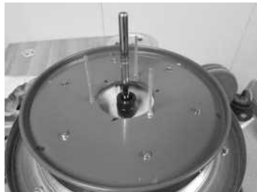
6. loosen the bolt of the hepa filter
