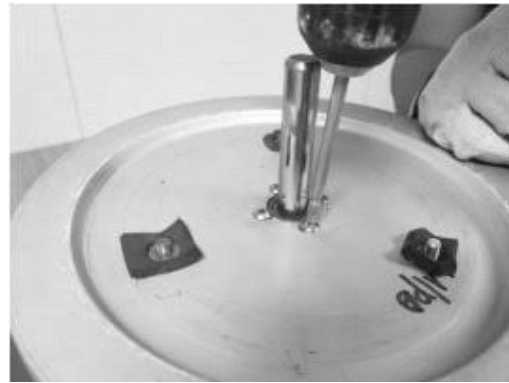
8. after replacement, assembly is reversed.
