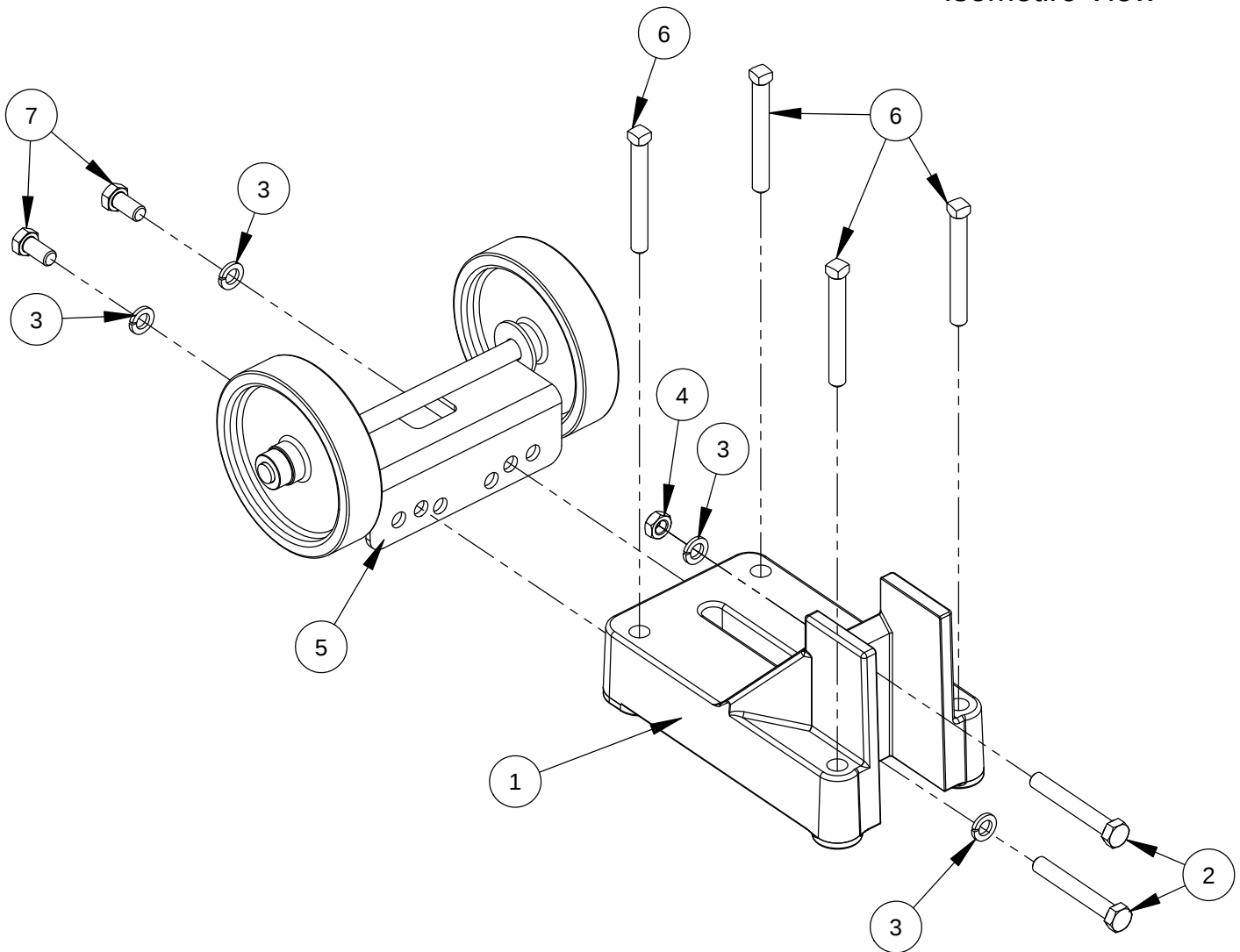
Isometirc View
