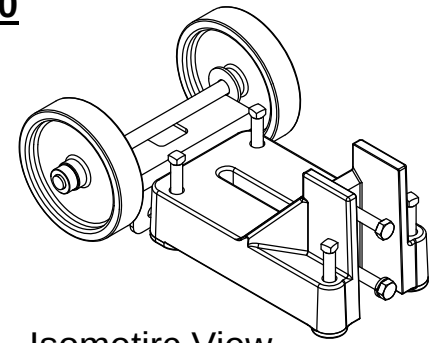
Isometirc View
